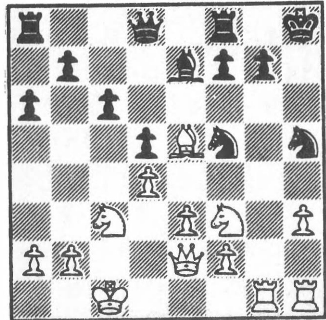
449 After 19...Nxf5
